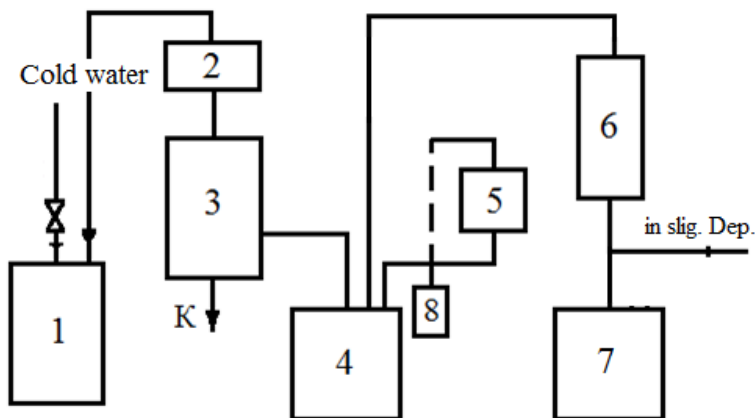
Figure 1 – Apparatus for preparing an adhesive formulation
